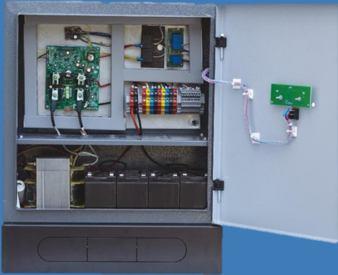
ARD Rescues Device With 4 Battery
